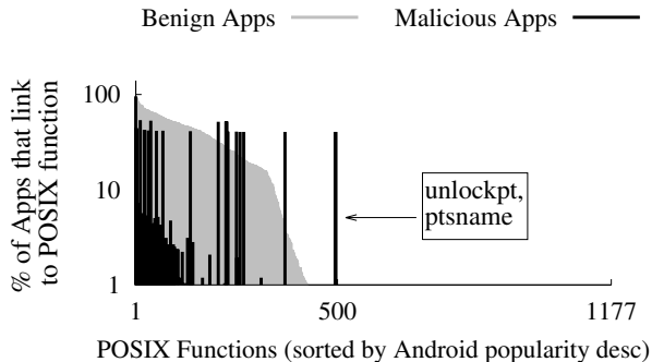
Figure 4: Popularity of POSIX in Benign vs. Malicious Apps. of bugs to survive over long periods. Our study reveals that this observation applies to POSIX and its implementation in Android. We find that the syslog function, a POSIX logging utility, is implemented by Android’s bionic libc, but the implementation is actually broken. Not only is there no syslog daemon process to which the syslog function would communicate, but the code also attempts to connect to a Unix domain socket named /dev/kmsg which in Android is actually a character device! (Incidentally, we found a similar side-effect in our prior work Cycada [7]: in iOS, the select system call, presumably also equally rarely used as in the OSes we study here, is buggy; its latency scales linearly with the number of file descriptors and the call fails to return when selecting on more than 250 descriptors.)
